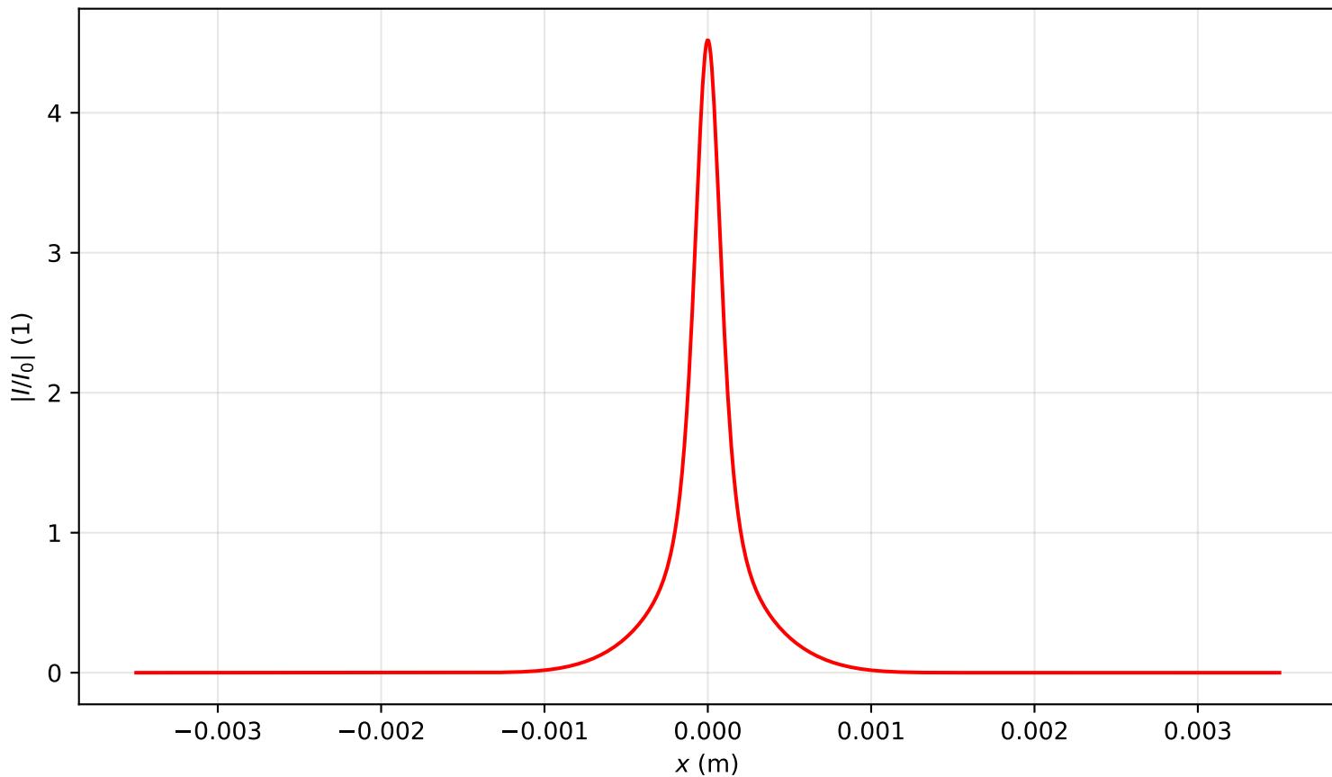
Intensity profile I(x, y = 0, z = 0.478)/I_0 , P_{in}=4.0P_{cr} , artificial time
